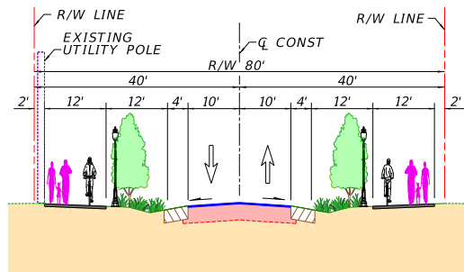
Typical Section of Proposed Improvements
